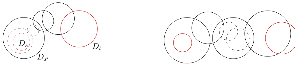
(a) Omitting the dashed disks and querying for s' instead of s still leads to a valid path to t .
